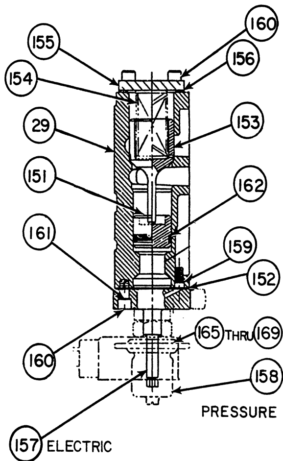
SUCTION CUTOFF CYLINDER HEAD ASSY.
