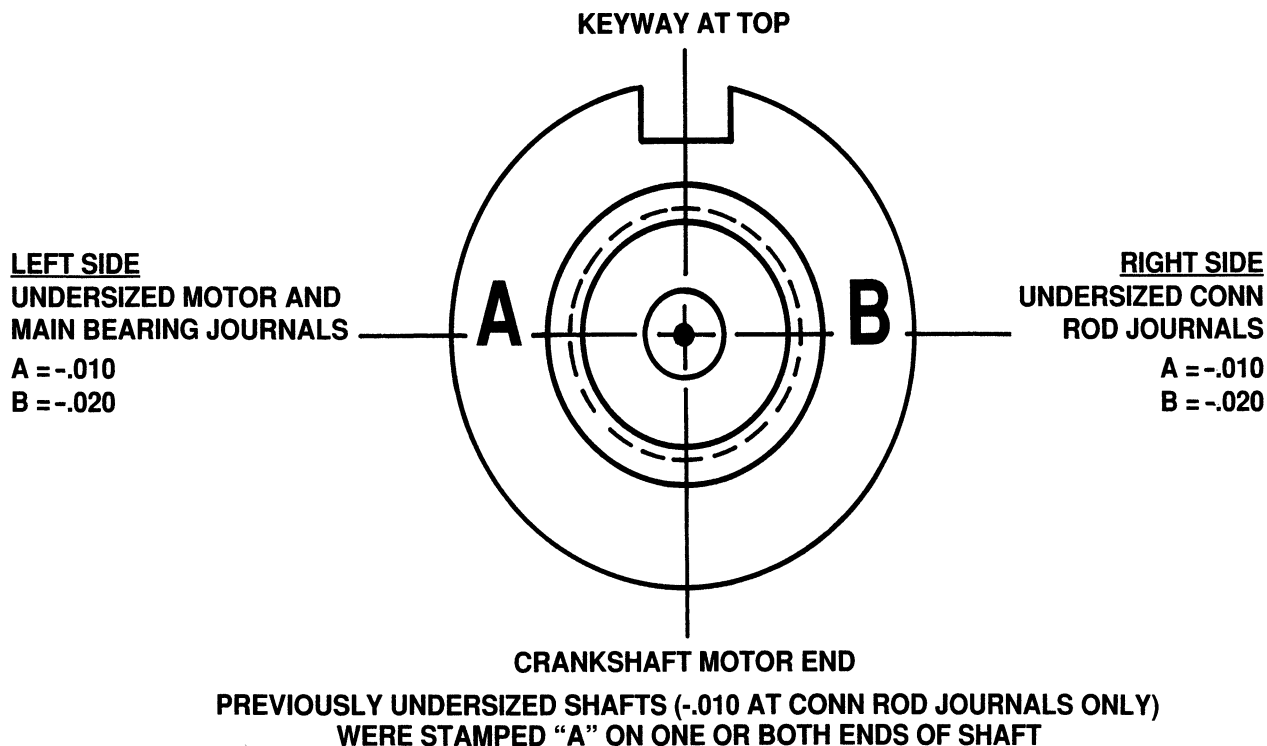
DETAIL "C"
