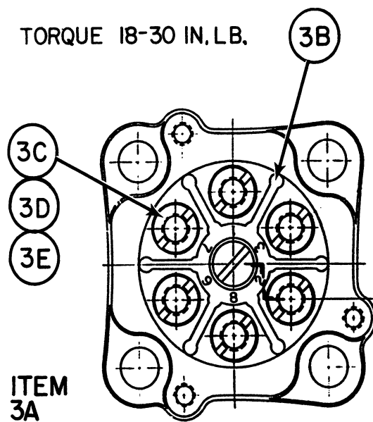
TERMINAL PLATE
