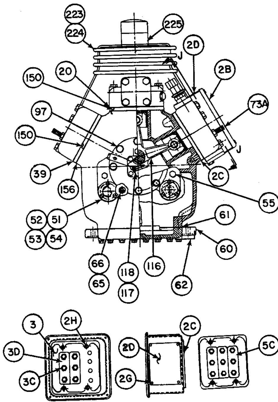
SECTION J-J
