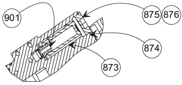
Section A - A, Oil Filter/Check Valve Asy
