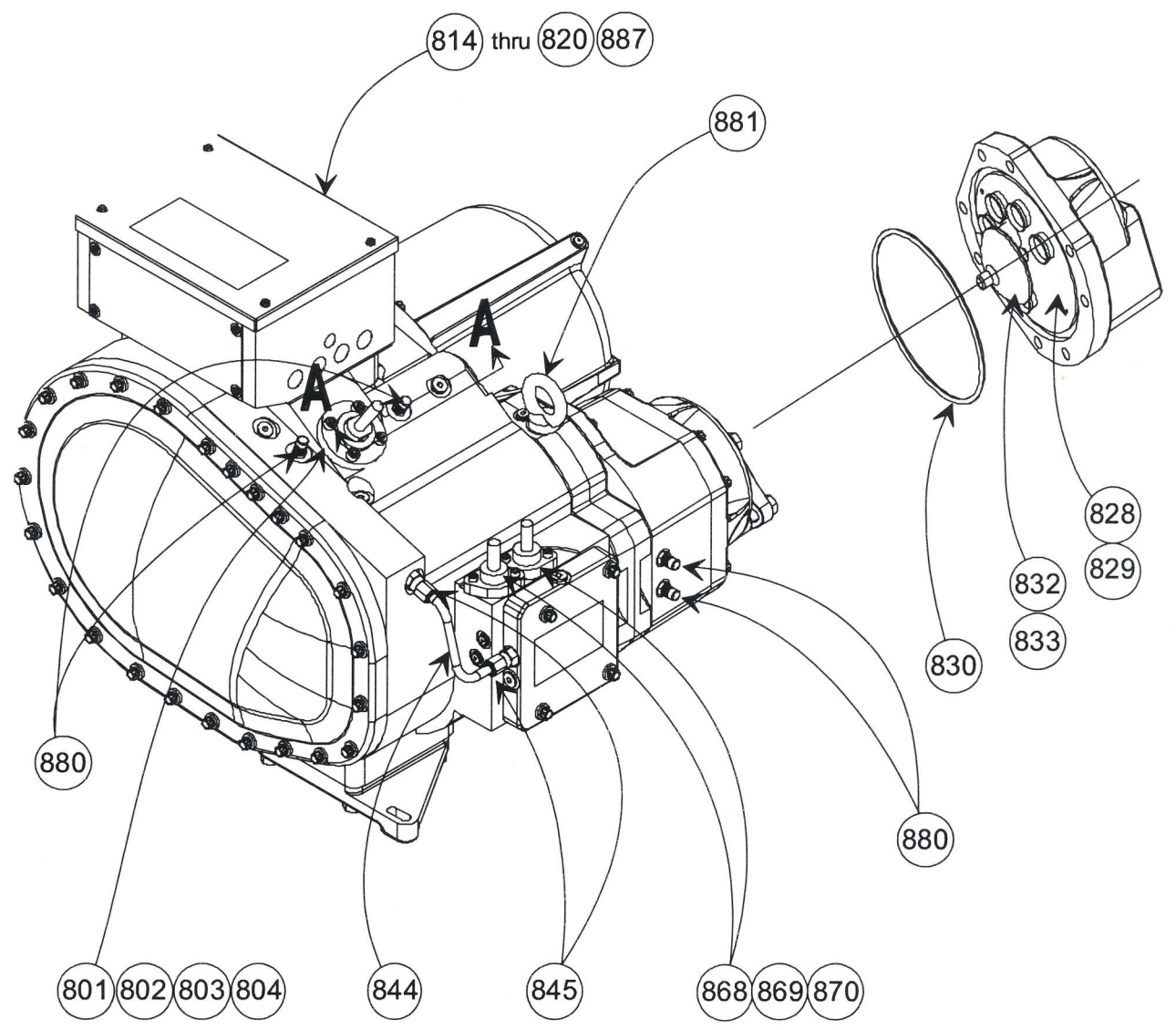
COMPRESSOR SERVICE KIT GROUP
