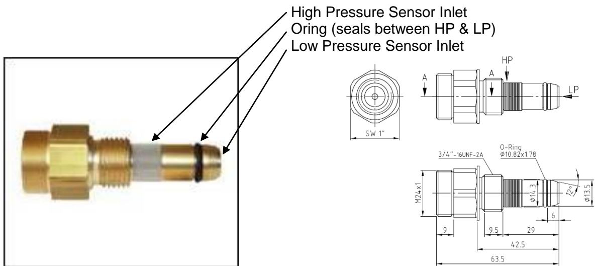
OPSS Sensor
