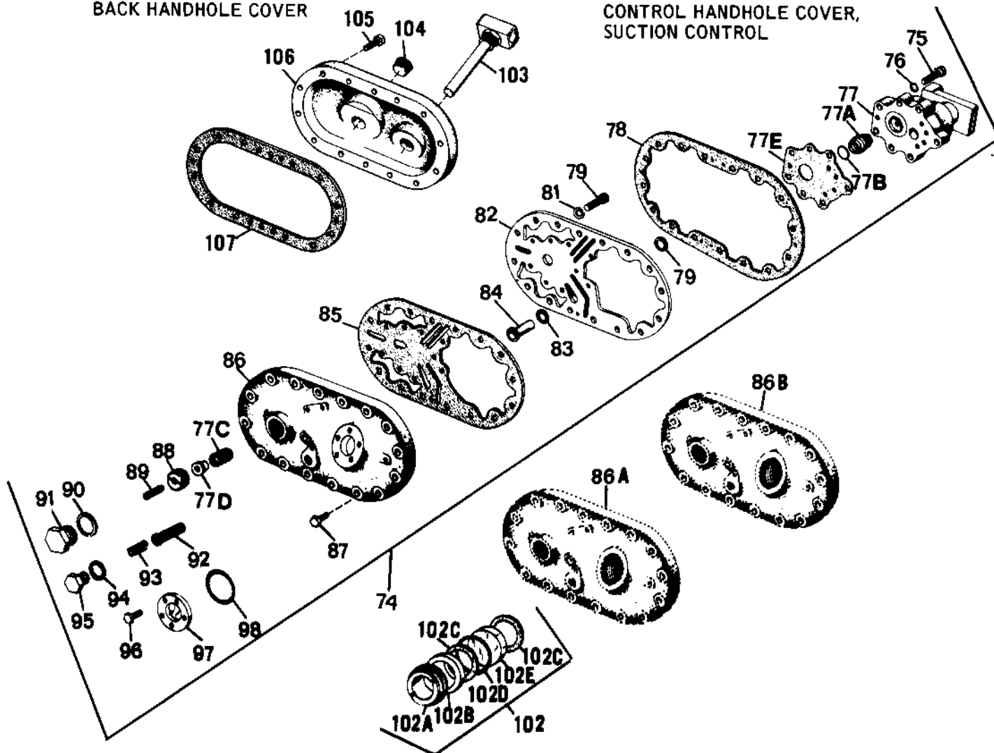
Control Handhole Cover Assembly (Cont.)
