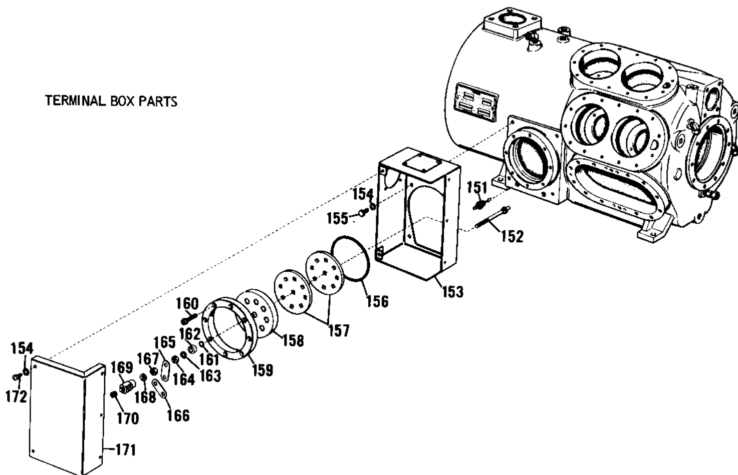
Terminal Box Parts
