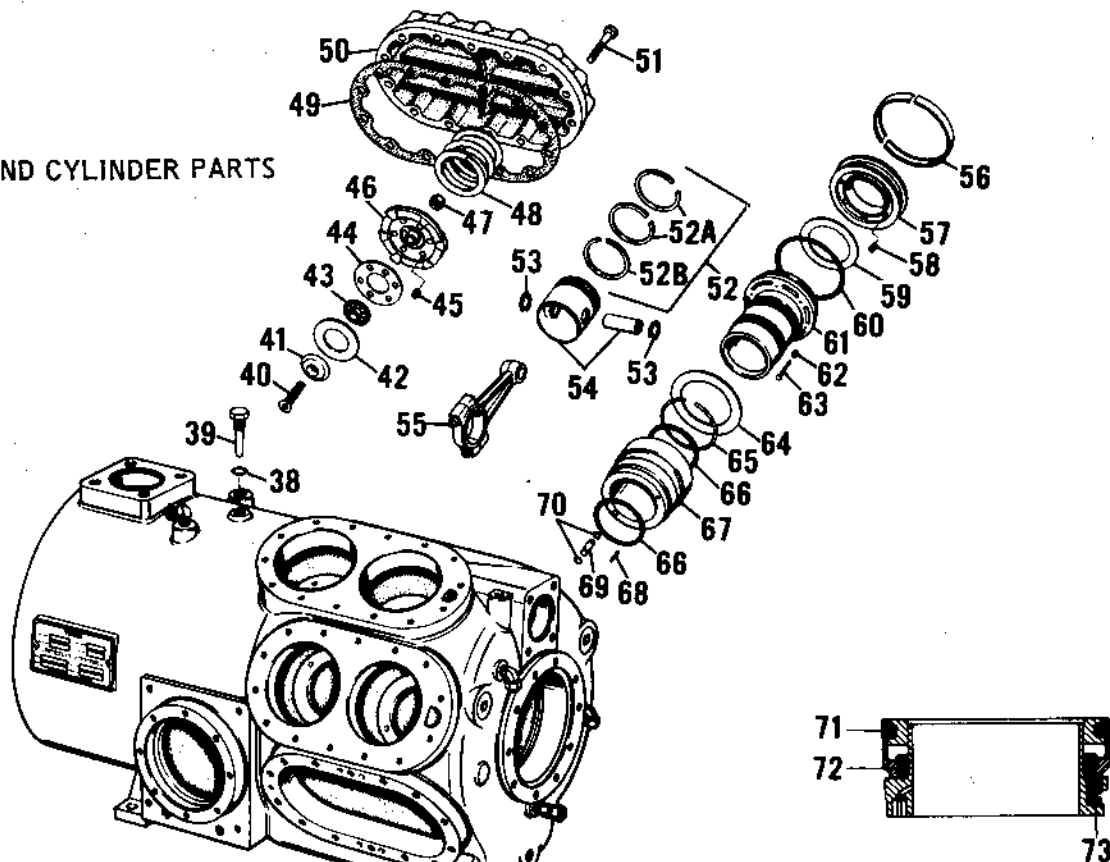
Head And Cylinder Parts
