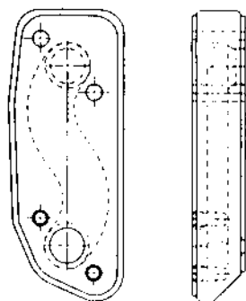
Adapter Plate
