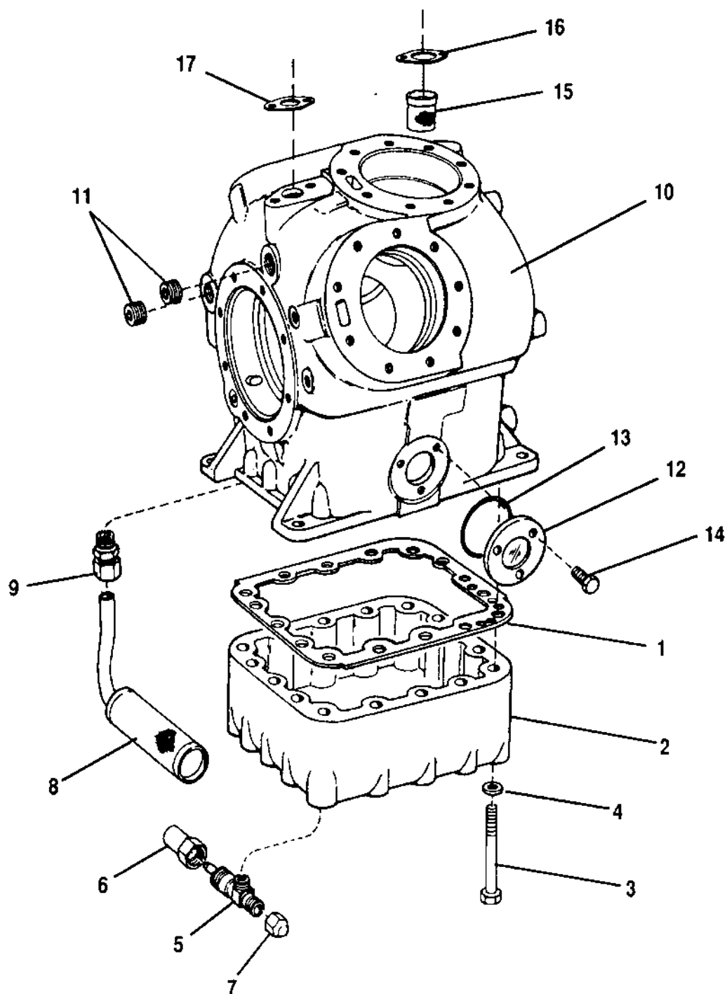
THERMOFILM GRID NO. 98A4 HAND HOLE COVER & OIL STRAINER (NON-UNLOADING MODELS)
