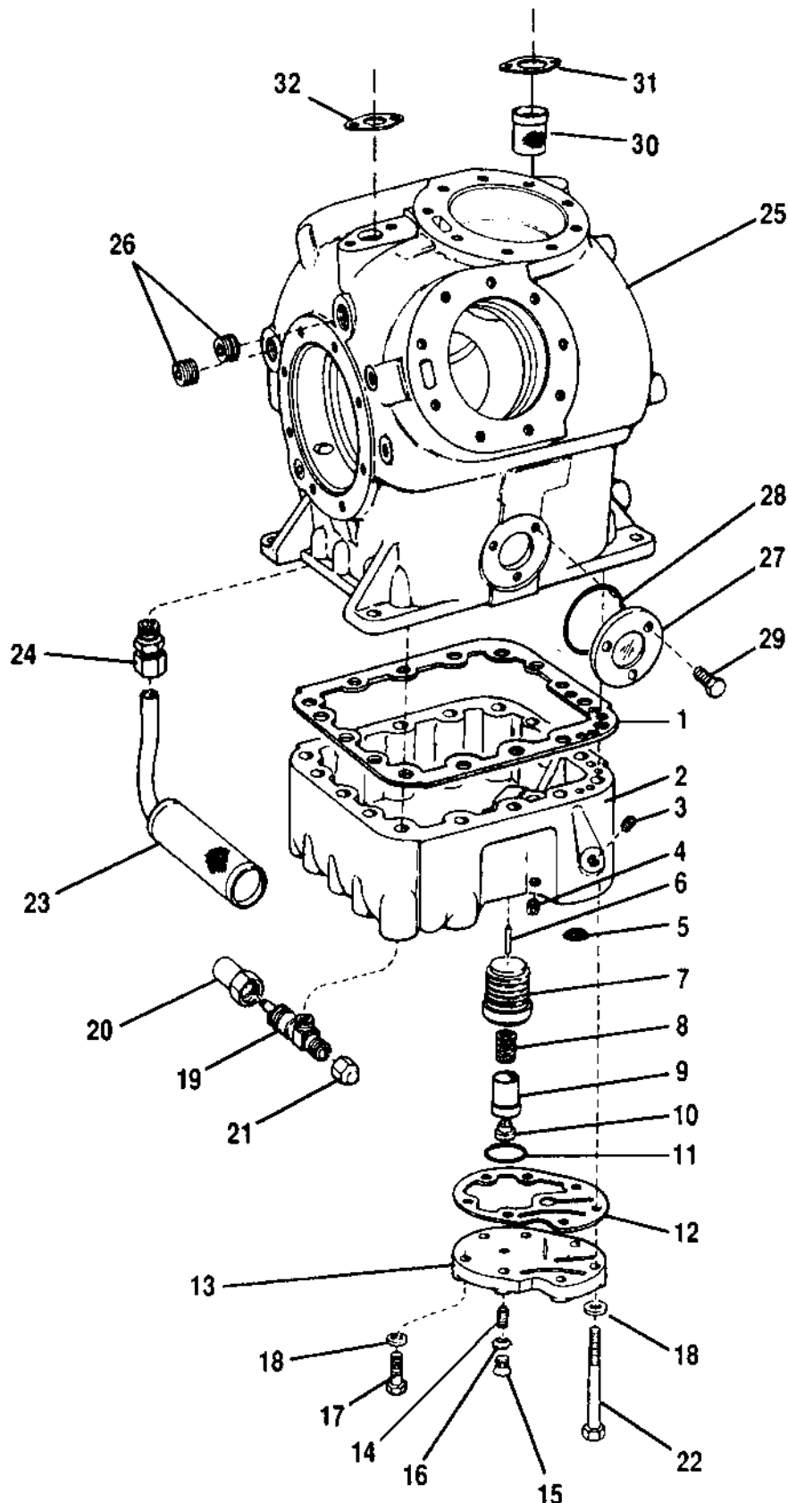
THERMOFILM GRID NO. 98A3 HAND HOLE COVER & OIL STRAINER GROUP (SUCTION UNLOADING MODELS)
