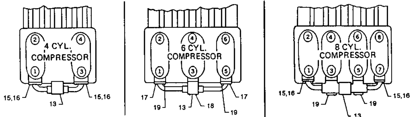
FIG. 5 - MANIFOLD ARRANGEMENTS
