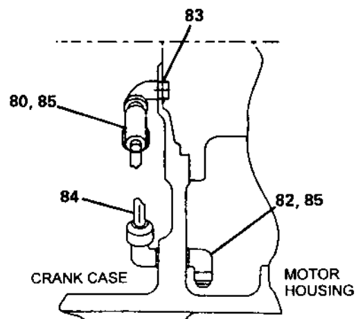
VIEW B-B
